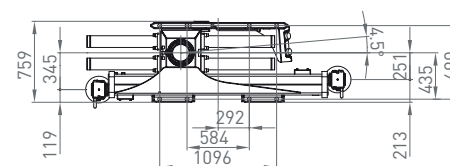
Sockel breit Crane base wide
