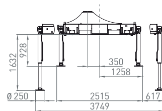
Sockel schmal Crane base small
