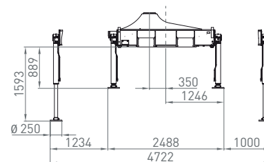
Sockel breit Crane base wide
