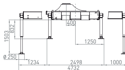
Socket Crane base
