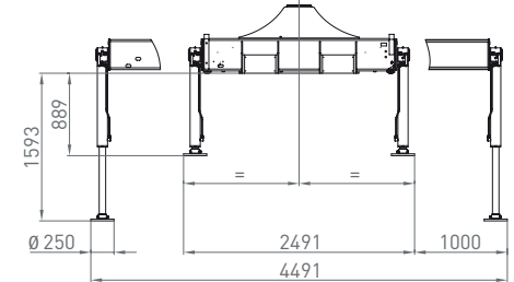
Socket wide Crane base wide
