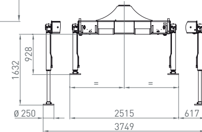
Socket small Crane base small
